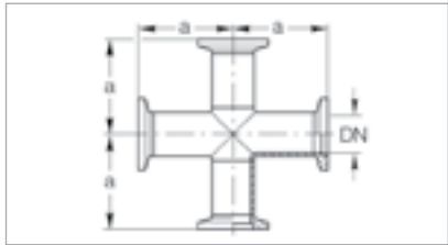
Dimensional drawing for the 4-way crosses
