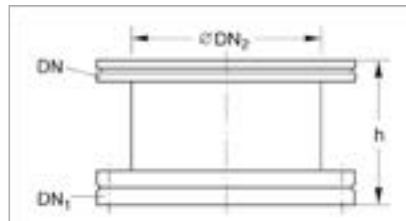
Dimensional drawing for the adaptors ISO-K – CF
