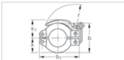
Dimensional drawing for the quick clamping rings
