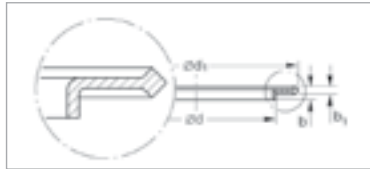
Dimensional drawing for O-rings
