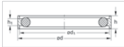
Dimensional drawing for the outer centering rings with O-ring
