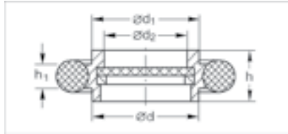
Dimensional drawing for the centering rings with O-ring
