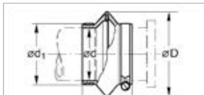
Dimensional drawing for the flexible compensation elements
