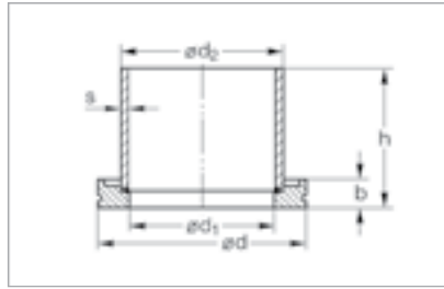
Dimensional drawing for the clamp flanges with tubulation
