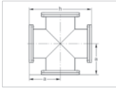
Dimensional drawing for the crosses
