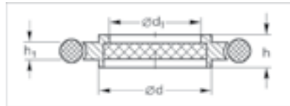
Dimensional drawing for the centering rings with sintered metal filter and O-ring
