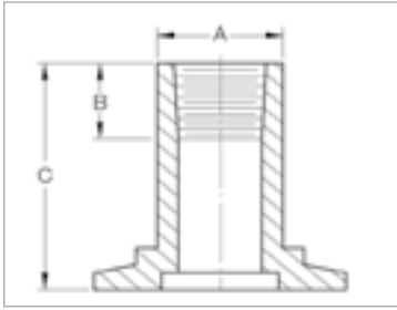
Dimensional drawing for the ISO-KF/NPT female adaptors
