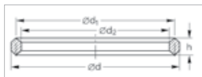
Dimensional drawing for the ultra sealing rings
