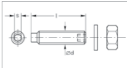
Dimensional drawing for the set screws, nuts and washers for CF flanges
