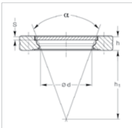
Dimensional drawing for CF observation windows
