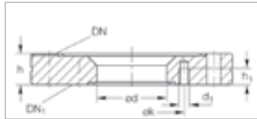
Dimensional drawing for the CF reducing flanges, fixed
