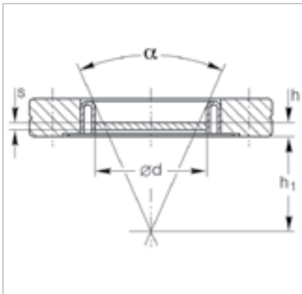
Dimensional drawing for the CF sapphire observation windows
