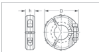
Dimensional drawing for the clamping collars for ultra sealing rings
