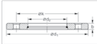
Dimensional drawing for collar flanges with retaining ring
