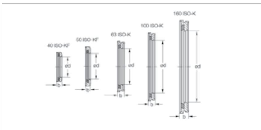
Window dimensions for the observation windows
