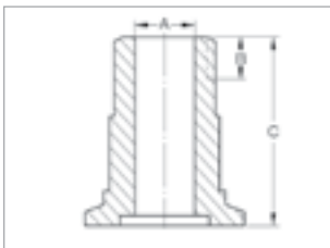
Dimensional drawing for the ISO-KF/NPT male adaptors
