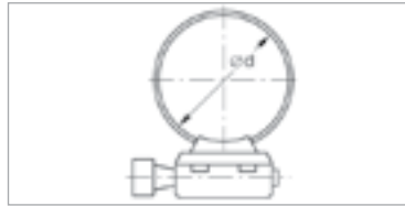
Dimensional drawing for the hose clamps
