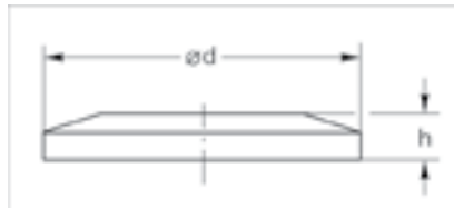
Dimensional drawing for the outer support rings
