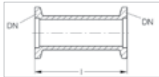
Dimensional drawing for the intermediate pieces
