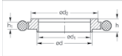
Dimensional drawing for the centering ring adaptors with O-ring
