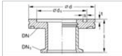
Dimensional drawing for the adaptors-reducer ISO-K – ISO-KF; left: aluminium; right: stainless steel
