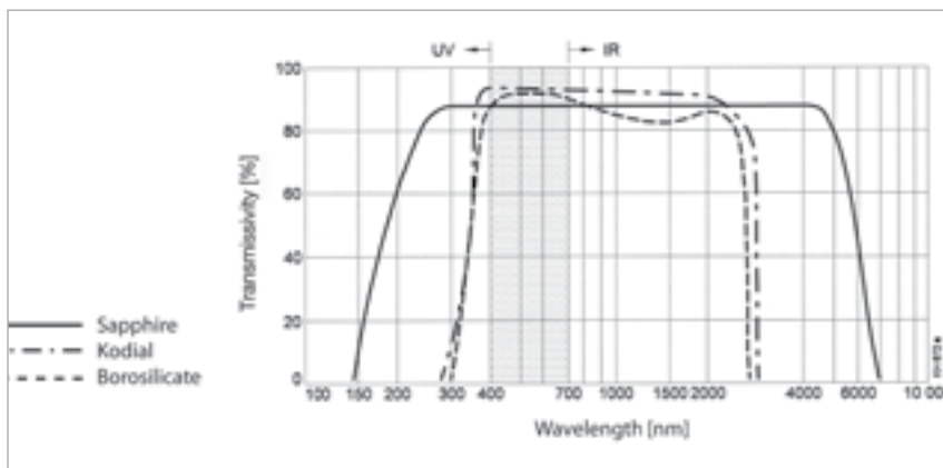
Optical transmissivity for the CF observation windows
