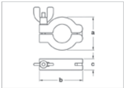
Dimensional drawing for the clamping rings
